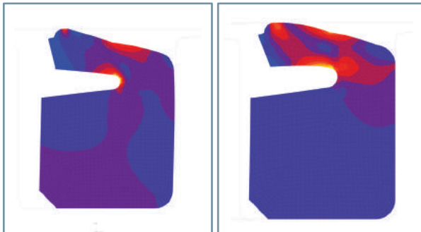
K59 @ 0 bar
